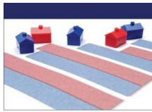
Pejman Bahramian Forecasting US Home Prices with Neural Network and Fuzzy Methods Combination and Single Forecasts
